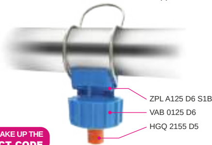
ZPL Double spring Better stability
