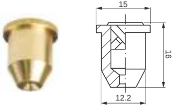
Above is outer shape of BX 1149 - BX 1372
