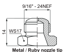
Metal / Ruby nozzle tip
