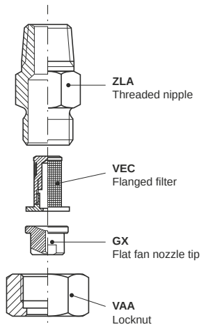
Assembly fittings
